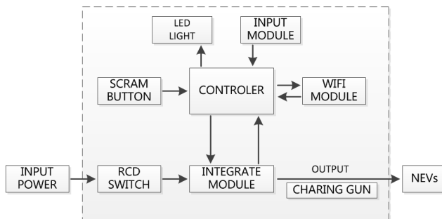
Figure 1-2 Functional principle block diagram
